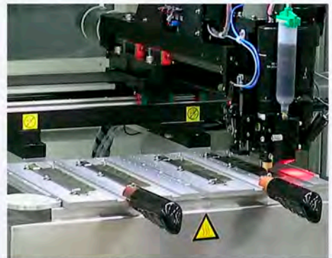
Manual Loading Tray & Heating Stage
